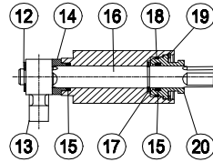
Stuffing Box Detail
