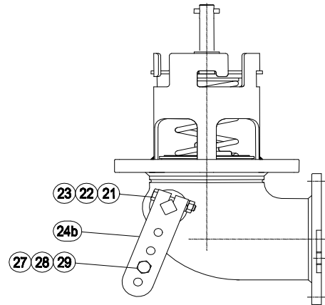
Cable Operated
